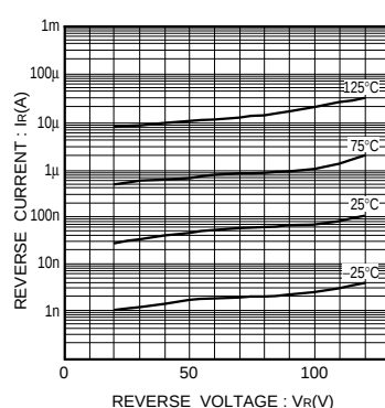
Fig.2 Reverse characteristics
