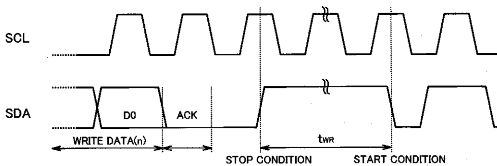
Fig.-9 WRITE CYCLE TIMING
