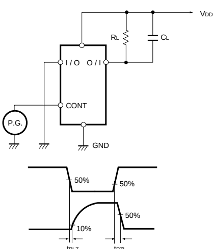
Fig. 2 (c) Propagation delay time (CONT to OUT)
