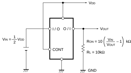
Fig. 1 (b) On resistance
