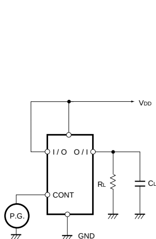
Fig. 2 (a) Propagation delay time (IN to OUT)
