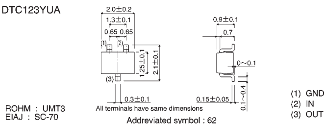
DTC123YKA
