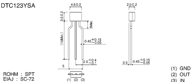
DTC123YSA
