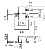
DTC124TE
