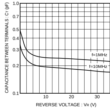
Fig.3 Capacitance between terminals characteristics (I)
