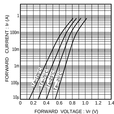
Fig. 1 Forward characteristics
