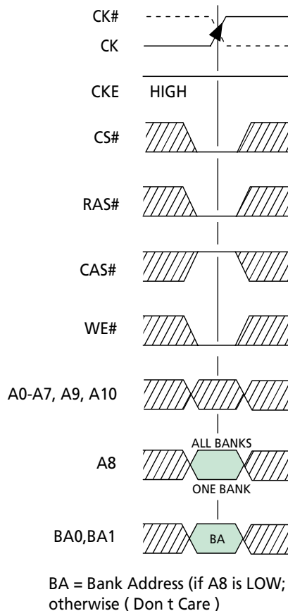
Figure 25 PRECHARGE Command
