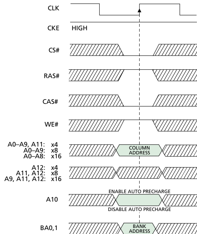
Figure 5 READ Command
