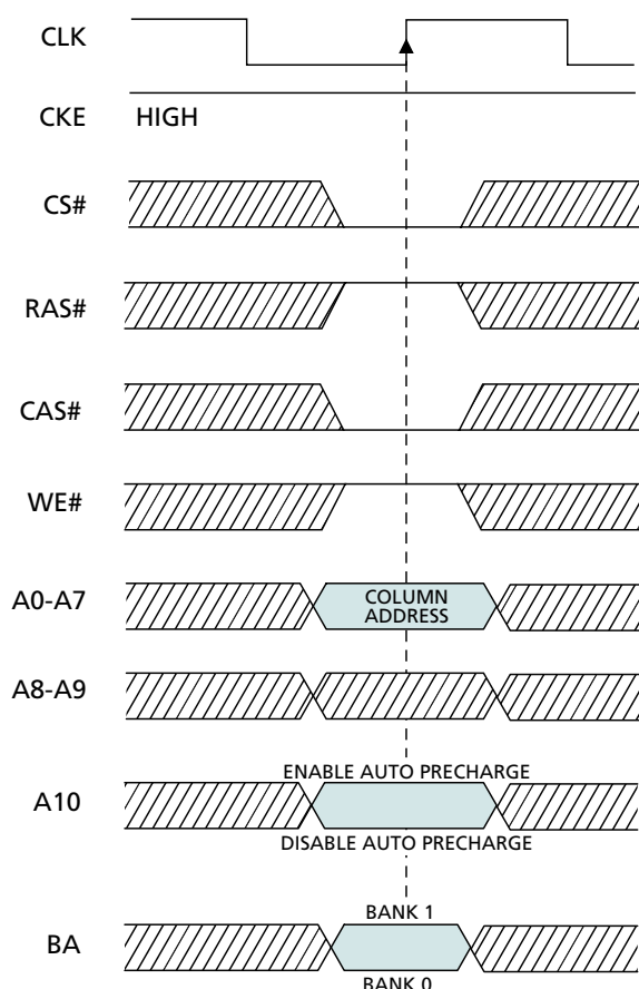
Figure 5 READ Command
