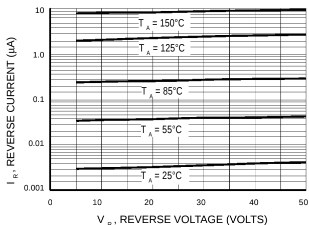
Figure 2. Leakage Current
