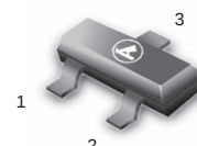
CASE 318, STYLE 11 SOT-23 (TO-236AB)
