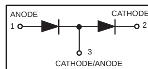
CASE 318, STYLE 11 SOT-23 (TO-236AB)
