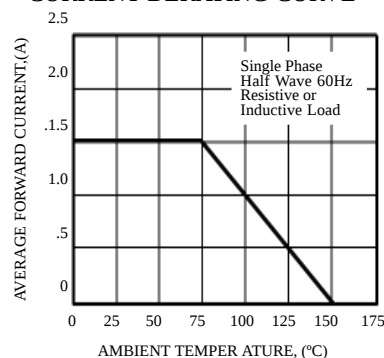
FIG. 2 – TYPICAL FORWARD CURRENT DERATING CURVE
