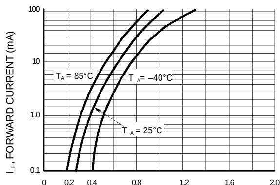
Figure 4. Forward Voltage
