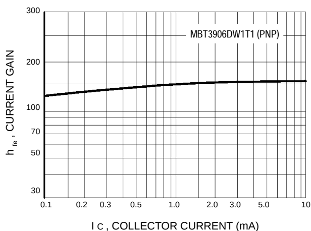
Figure 27. Current Gain
