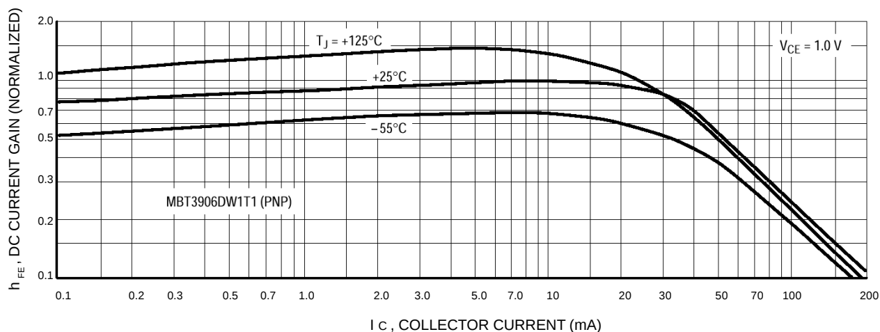
Figure 31. DC Current Gain
