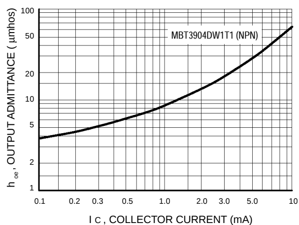
Figure 12. Output Admittance
