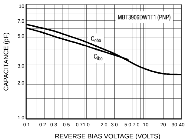
Figure 21. Capacitance
