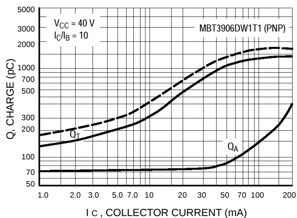
Figure 22. Charge Data
