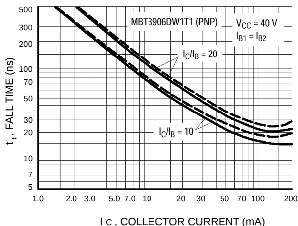
Figure 24. Fall Time
