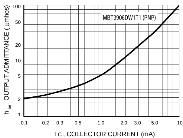
Figure 28. Output Admittance
