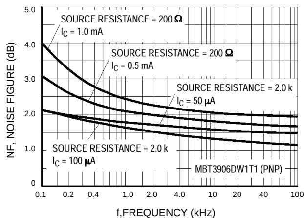
Figure 25. Noise Figure
