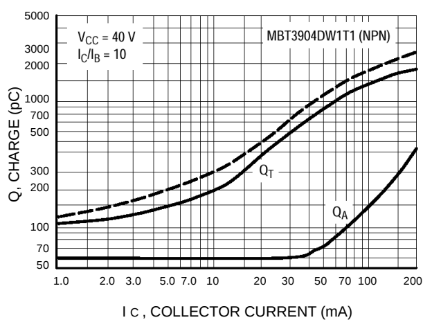
Figure 4. Charge Data
