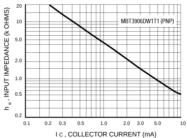
Figure 29. Input Impedance
