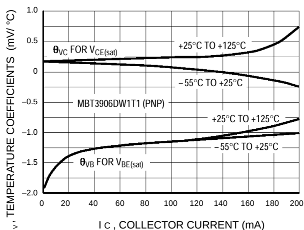
Figure 34. Temperature Coefficients
