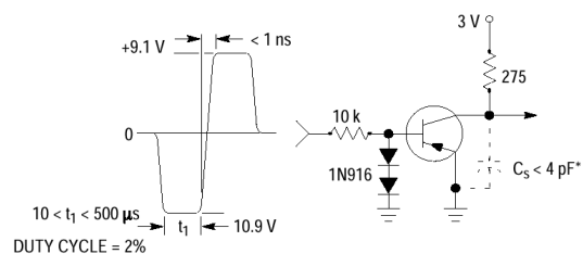
Figure 20. Storage and Fall Time Equivalent Test Circuit
