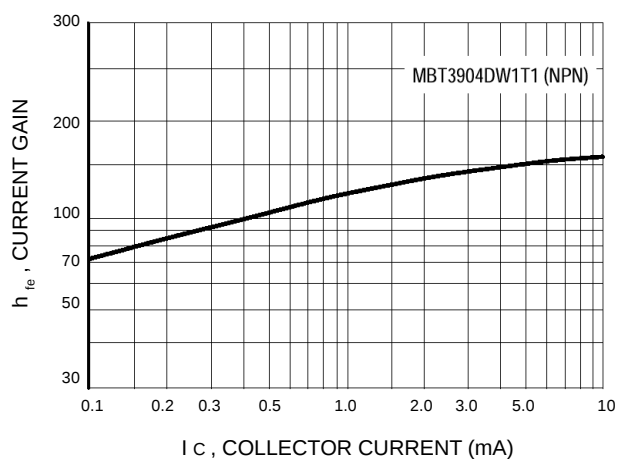
Figure 11. Current Gain
