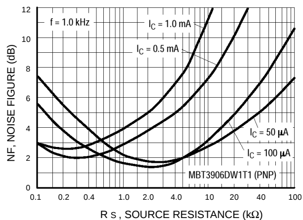
Figure 26. Noise Figure
