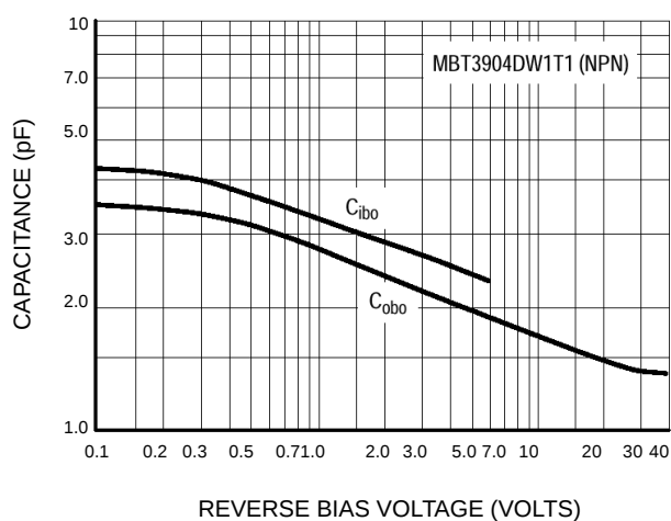
Figure 3. Capacitance
