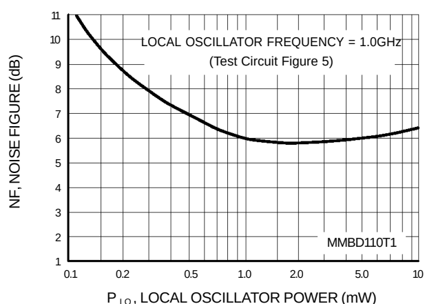
Figure 4. Noise Figure
