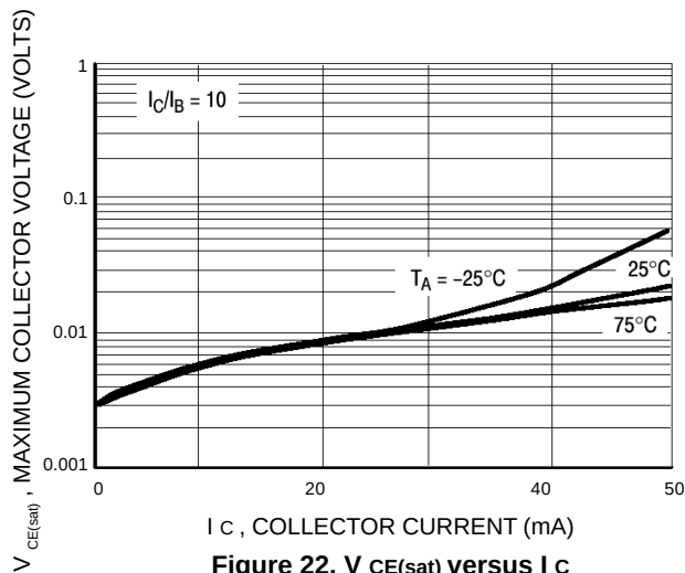
Figure 22. V_{CE(sat)} versus I_C
