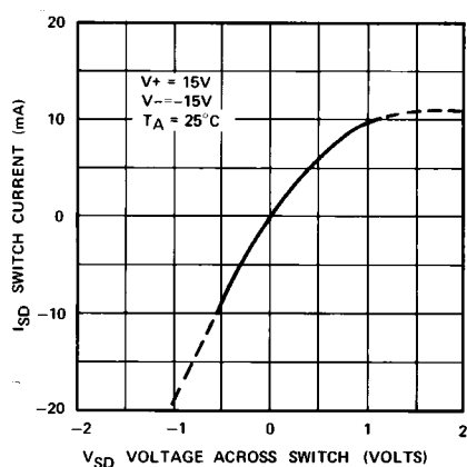
Switch Current vs. Voltage
