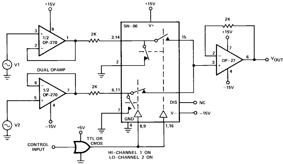
High Off Isolation Selector Switch (Shunt-Series Switch)
