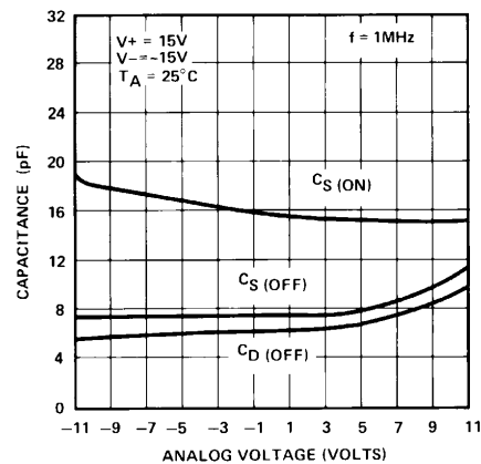
Switch Capacitance vs. Analog Voltage
