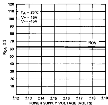
"ON" Resistance vs. Power Supply Voltage
