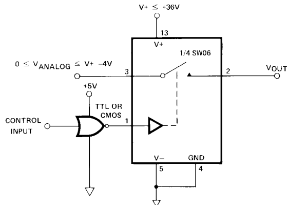
Operation from Single Positive Power Supply
