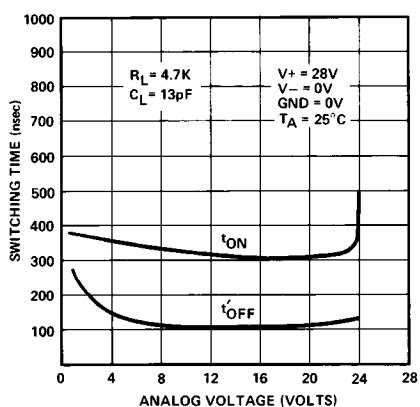
Switching Time vs. Supply Voltage
