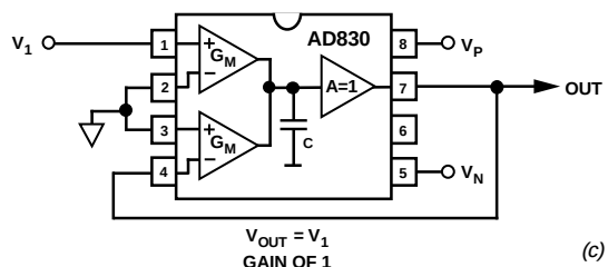
Figure 16. Connection Diagrams
