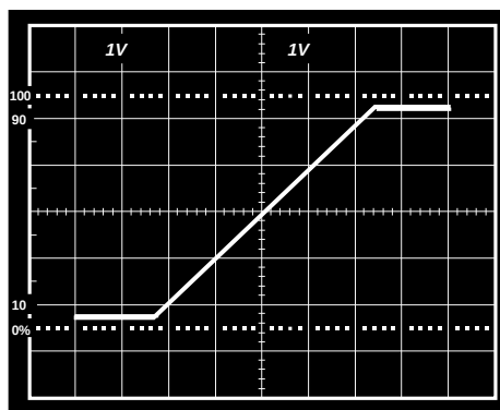
Figure 25. Clipping Behavior
