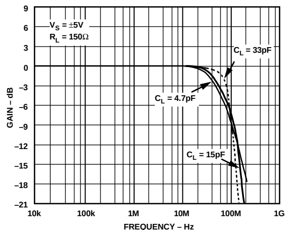
Closed-Loop Gain vs. Frequency, Gain = +1
