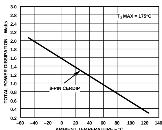
Maximum Power Dissipation vs. Temperature, Cerdip Package
