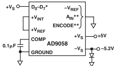
Burn-In Connections
