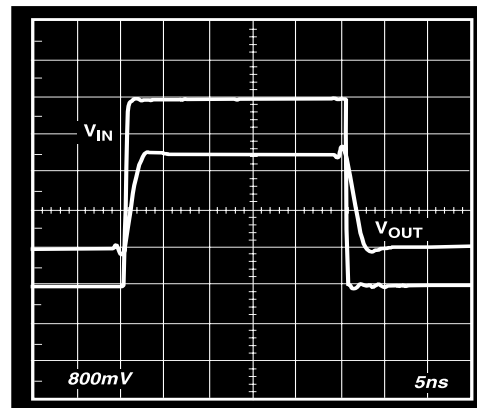
Figure 13. Clamped Large Signal Transient Response (2× Overdrive); V_O = 2\text{ V p-p} , G = +2 , R_F = R_{IN} = 274\ \Omega , V_H = +0.5\text{ V} , V_L = -0.5\text{ V}
