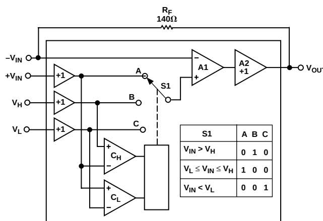
Figure 72. AD8036/AD8037 Clamp Amp System
