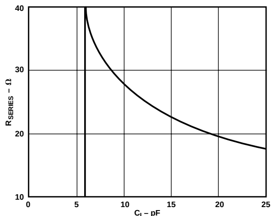
Figure 71. Recommended R_{\text{SERIES}} vs. Capacitive Load
