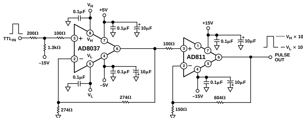
Figure 77. Programmable Pulse Generator
