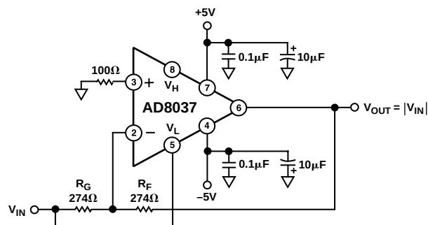
Figure 78. Full-Wave Rectifier
