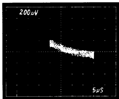
Figure 12. Dielectric Absorption
