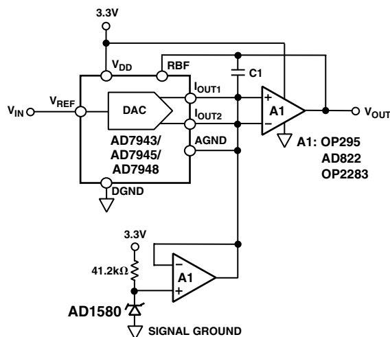
Figure 17. Single-Supply System
