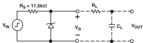
Figure 11b. Turn-On, Settling, and Transient Test Circuit
