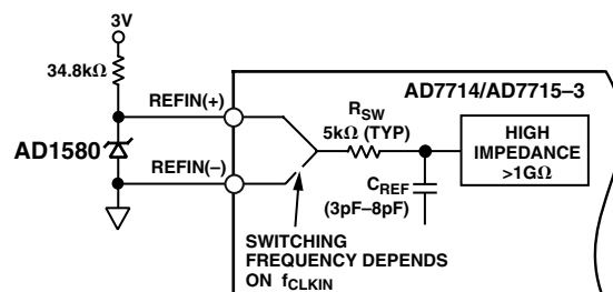
Figure 16. Reference Circuit for the AD7714/AD7715-3
