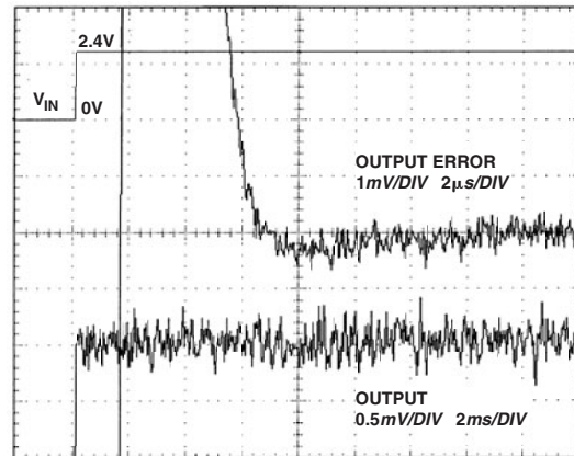
Figure 12. Turn-On Settling
