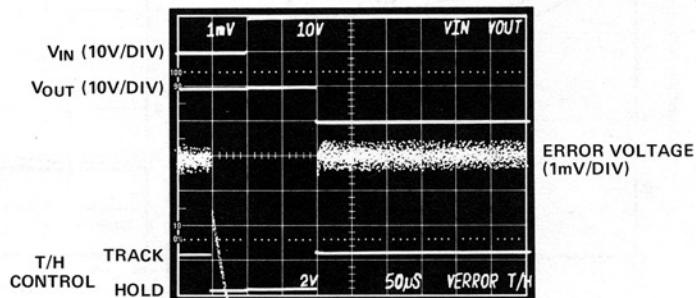
Figure 11a. Acquisition Time after 100µs in the Hold Mode. The AD389 Shows no "Thermal Tail".
