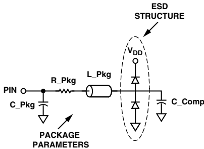
Figure 5. Input Buffer
