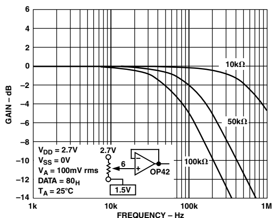
TPC 15. -3 dB Bandwidth
