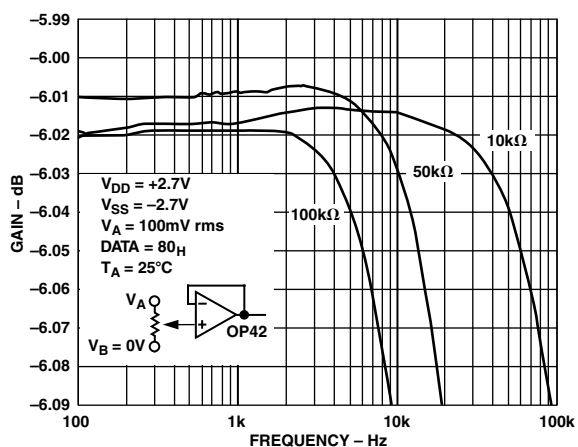
TPC 16. Normalized Gain Flatness vs. Frequency
