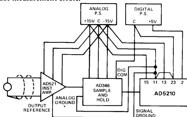
*IF INDEPENDENT, OTHERWISE RETURN AMPLIFIER REFERENCE TO MECCA AT ANALOG P.S. COMMON Figure 5. Basic Grounding Practice
