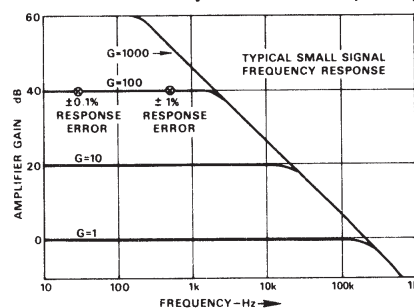
Figure 6. Small Signal Frequency Response (-3dB)
