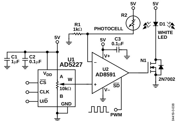
Figure 36. Automatic LCD Panel Backlight Control
