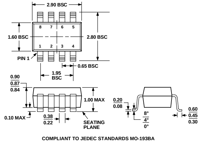
Figure 40. 8-Lead Small Outline Transistor Package TSOT-8 [Thin SOT-23-8] (UJ-8) Dimensions shown in millimeters
