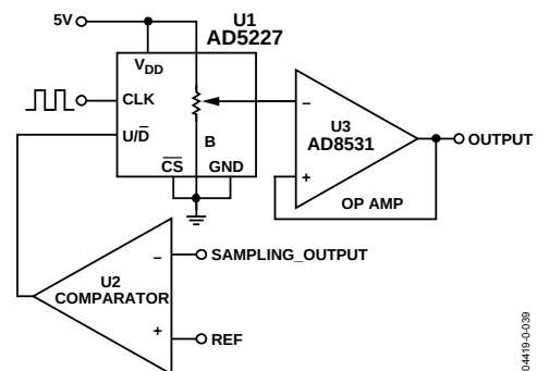
Figure 37. 6-Bit Controller
