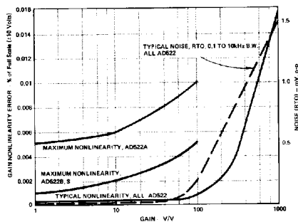
Figure 4. Gain Nonlinearity and Noise (RTO) vs. Gain
