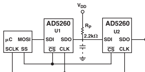
Figure 10. Daisy-Chain Configuration
