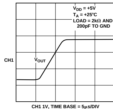
Figure 16. Half-Scale Settling (1/4 to 3/4 Scale Code Charge)
