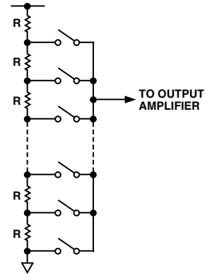
Figure 5. Resistor String
