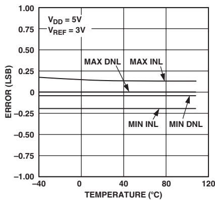
TPC 8. AD5302 INL Error and DNL Error vs. Temperature
