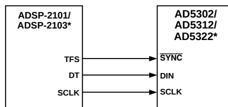
Figure 32. AD5302/AD5312/AD5322 to ADSP-2101/ADSP-2103 Interface
