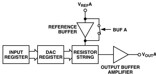
Figure 27. Single DAC Channel Architecture
