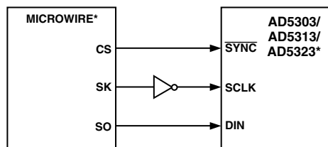
Figure 36. AD5303/AD5313/AD5323 to MICROWIRE Interface
