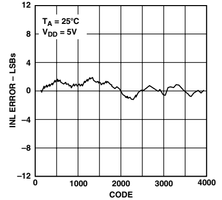
Figure 6. AD5324 Typical INL Plot
