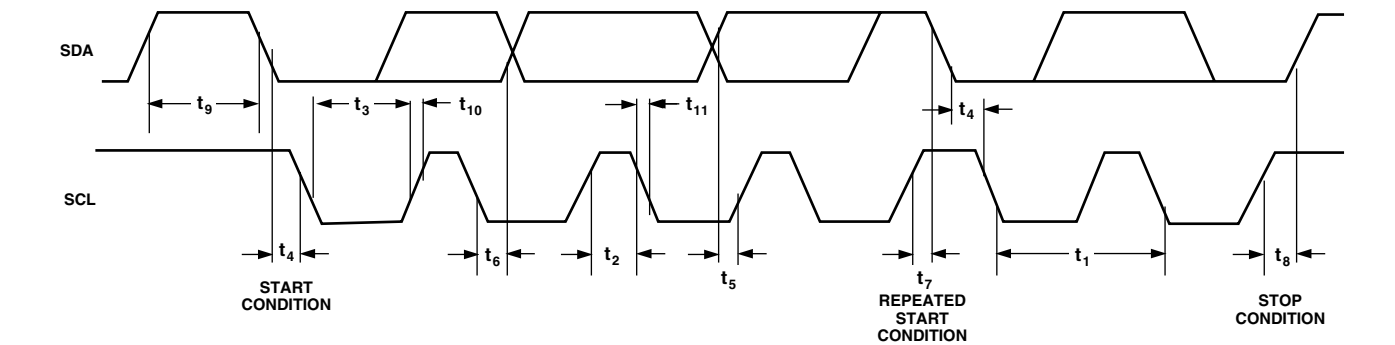
Figure 1. Two-Wire Serial Interface Timing Diagram
