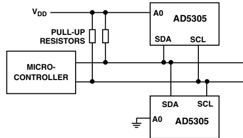
Figure 36. Multiple AD5305 Devices on One Bus
