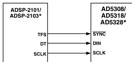
Figure 11. ADSP-2101/ADSP-2103 to AD5308/AD5318/AD5328 Interface
