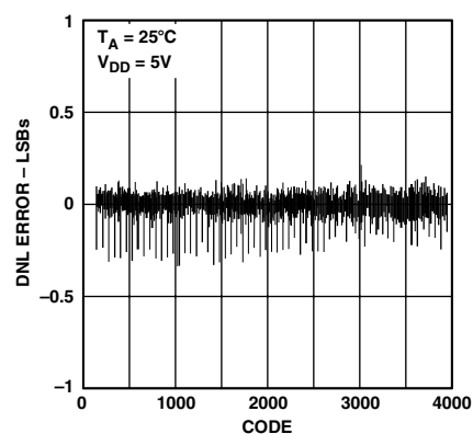
TPC 6. AD5328 Typical DNL Plot
