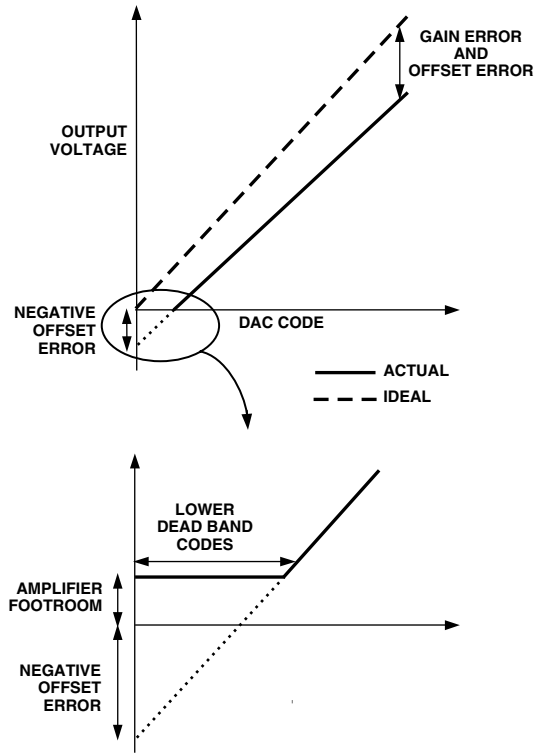
Figure 2. Transfer Function with Negative Offset ( V_{REF} = V_{DD} )
