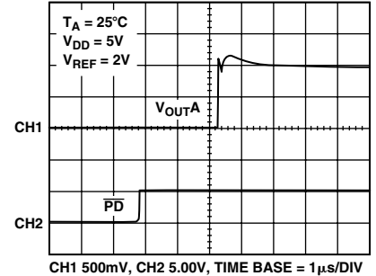
TPC 18. Exiting Power-Down to Midscale
