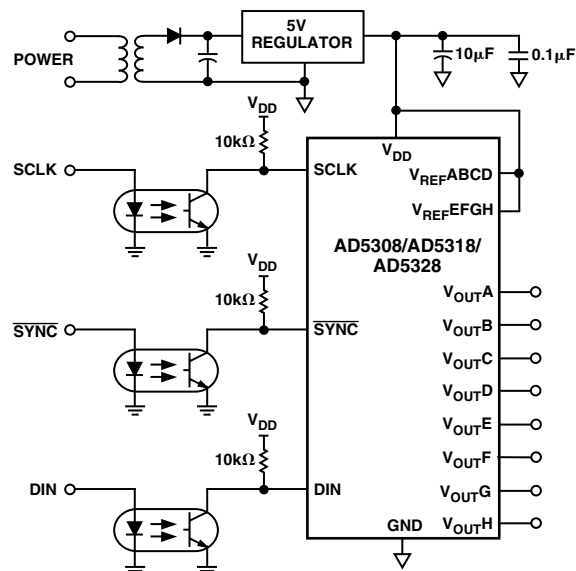
Figure 17. AD5308/AD5318/AD5328 in an Opto-Isolated Interface
