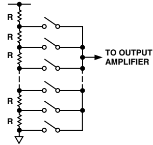
Figure 5. Resistor String
