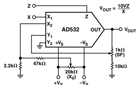
Figure 13. Divider Connection
