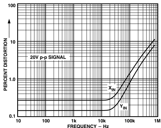
Figure 4. Percent Distortion vs. Frequency
