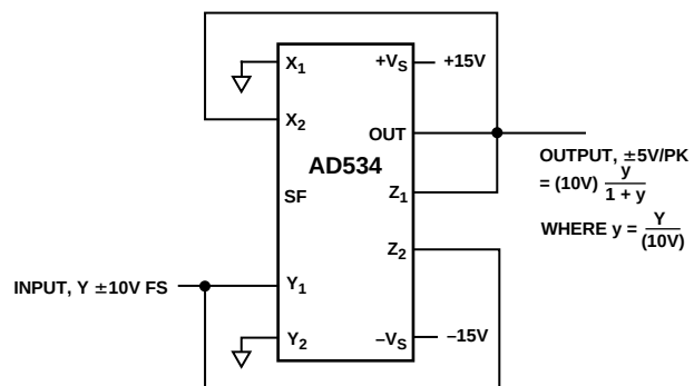
Figure 13. Bridge-Linearization Function
