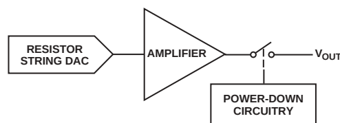
Figure 9. Output Stage During Power-Down
