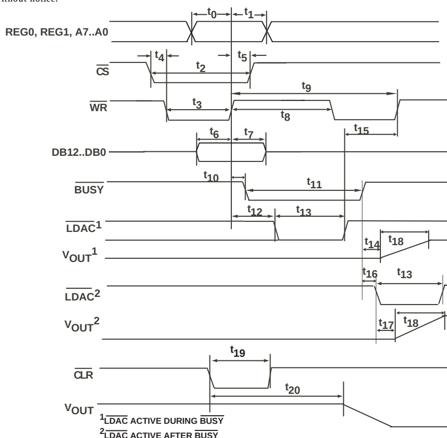
Figure 2. Parallel Interface Timing Diagram
