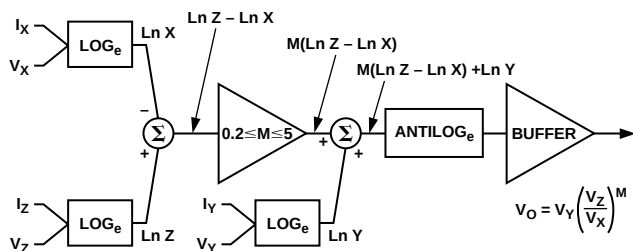
Figure 10. Model Circuit
