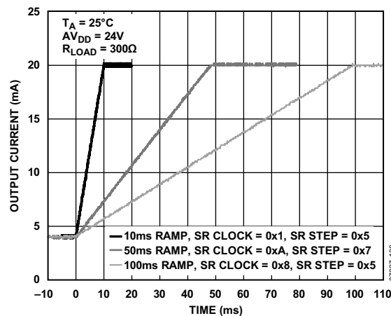
Figure 43. Output Current Slewing Under Control of the Digital Slew Rate Control Feature
