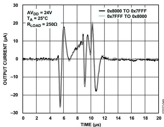
Figure 35. Digital-to-Analog Glitch
