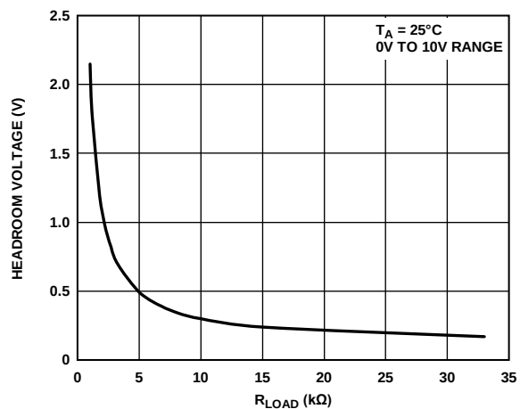
Figure 34. V_{OUT} Headroom
