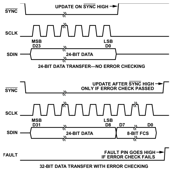
Figure 41. PEC Timing
