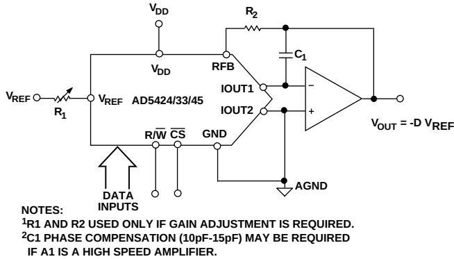
Figure 4. Unipolar Operation
