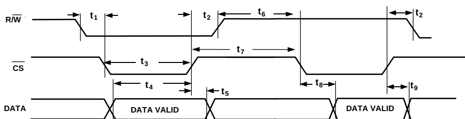
Figure 1. Timing Diagram.
