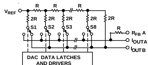
Figure 3. Simplified Ladder
