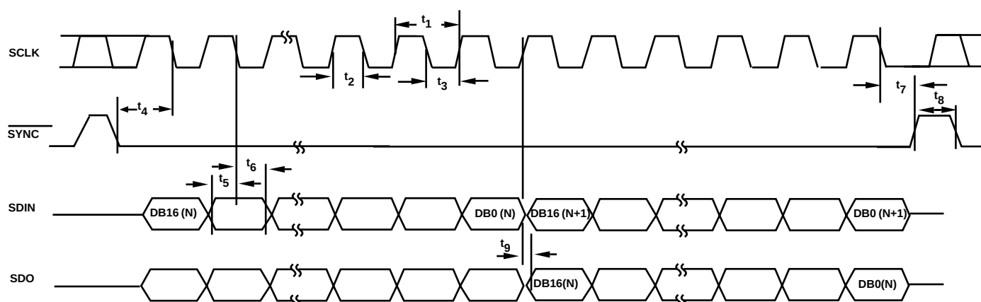
Figure 1. Stand Alone Mode Timing Diagram.
