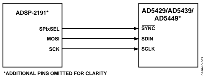
Figure 47. ADSP-2191 SPI to AD5429/AD5439/AD5449 Interface
