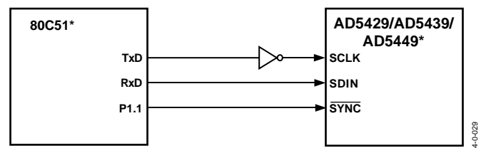
Figure 49. 80C51/80L51 to AD5429/AD5439/AD5449 Interface
