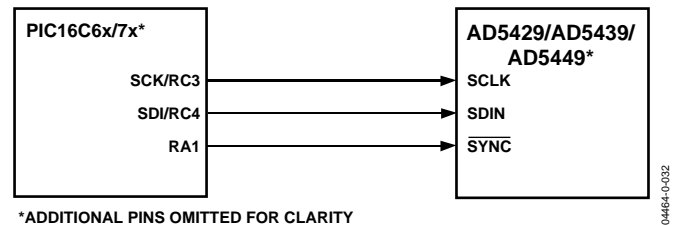
Figure 52. PIC16C6x/7x to AD5429/AD5439/AD5449 Interface
