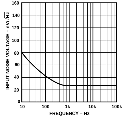
Figure 17. Input Noise Voltage vs. Frequency
